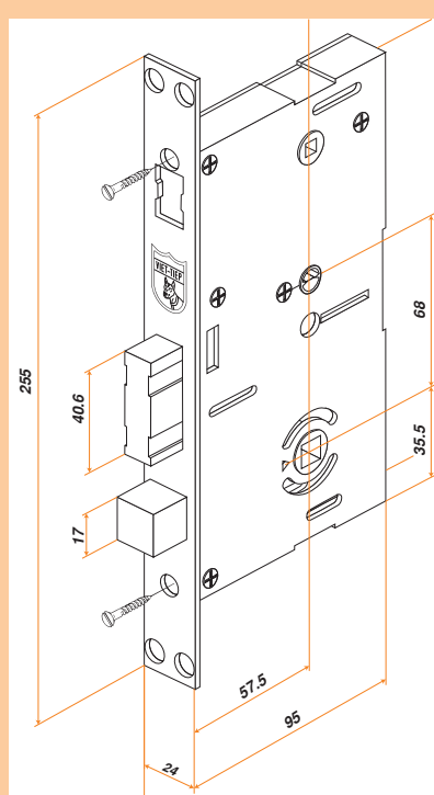
Hộp khóa 28285 Lock case 28285
