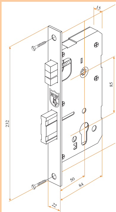
Hộp khóa 28286 Lock body 28286
