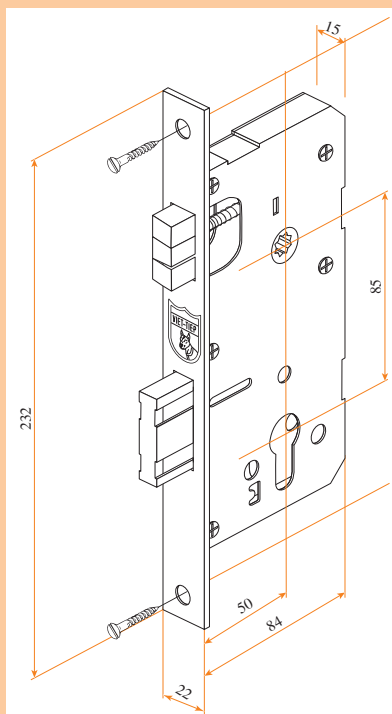
Hộp khóa 28286 Lock case 28286
