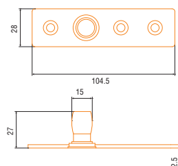
Ngõng cửa 11075 (Door tenon-like hinge)
